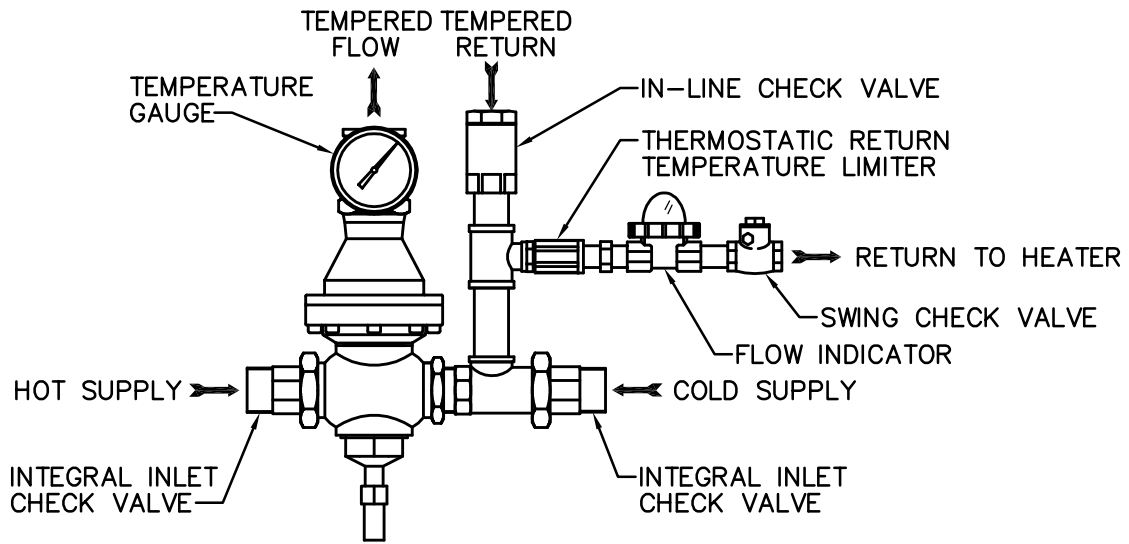
Factory Supplied TMV Piping Connections and Components
